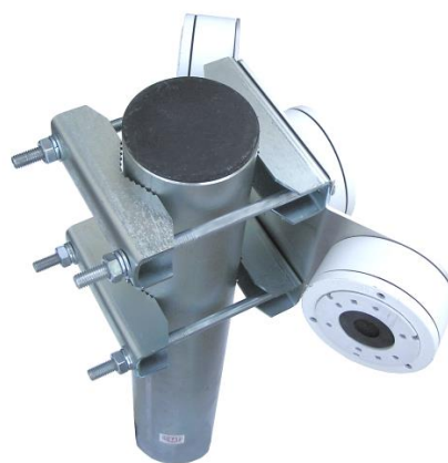
HIK100E TRIO + 2x 2Z5M + 3x DS-1280ZJ-XS montáž na trubku (Ø 90mm)
